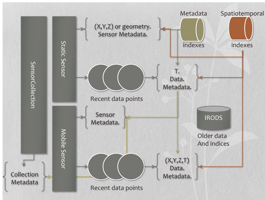
Figure 4 SensorCollection architecture
