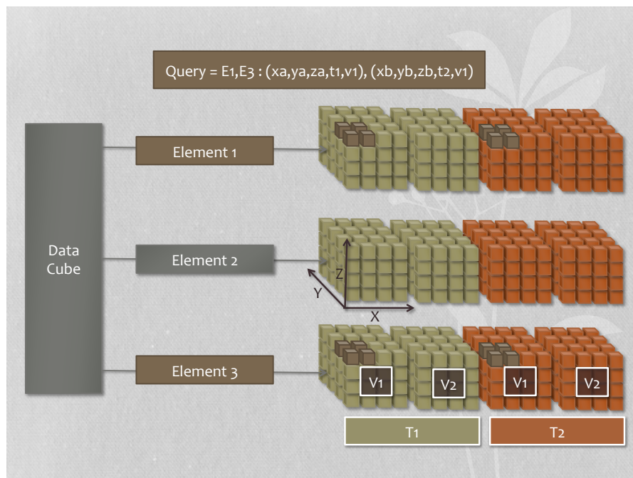
Figure 2; DataCube architecture and query behaviour
