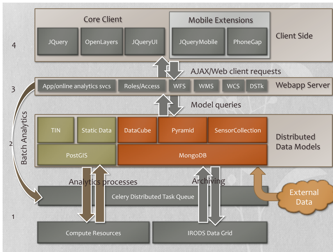
Figure 1 Architecture of Geoanalytics
