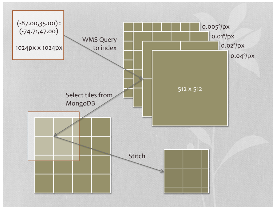
Figure 3 Pyramid architecture and query behaviour
