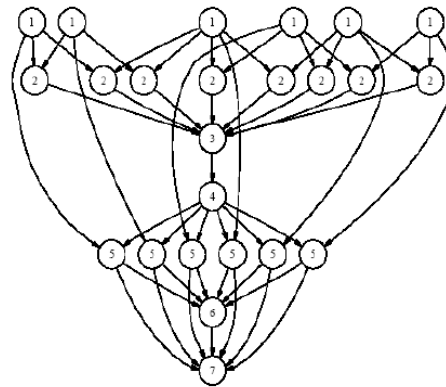
Fig. 3. A Small Montage Workflow
