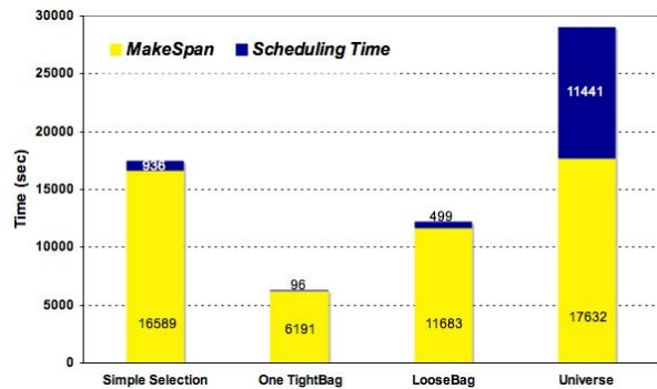
Fig. 9. Average MakeSpan and Scheduling Time for DAGs with CCR=10
