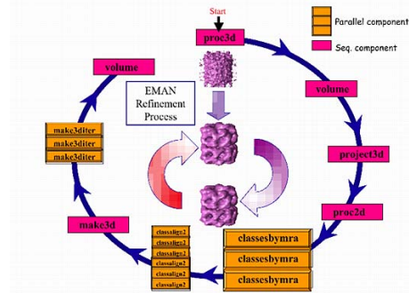
Fig. 2. EMAN Refinement Workflow
