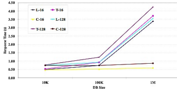
Fig. 1. Time to complete vgDL queries with vgES.
